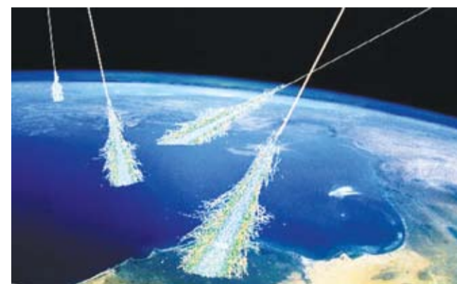
An artist's illustration of cosmic rays, just one form of cosmic radiation, striking molecules in the Earth's upper atmosphere producing cascades of lighter particles called an air-shower which then interact with the biosphere.
