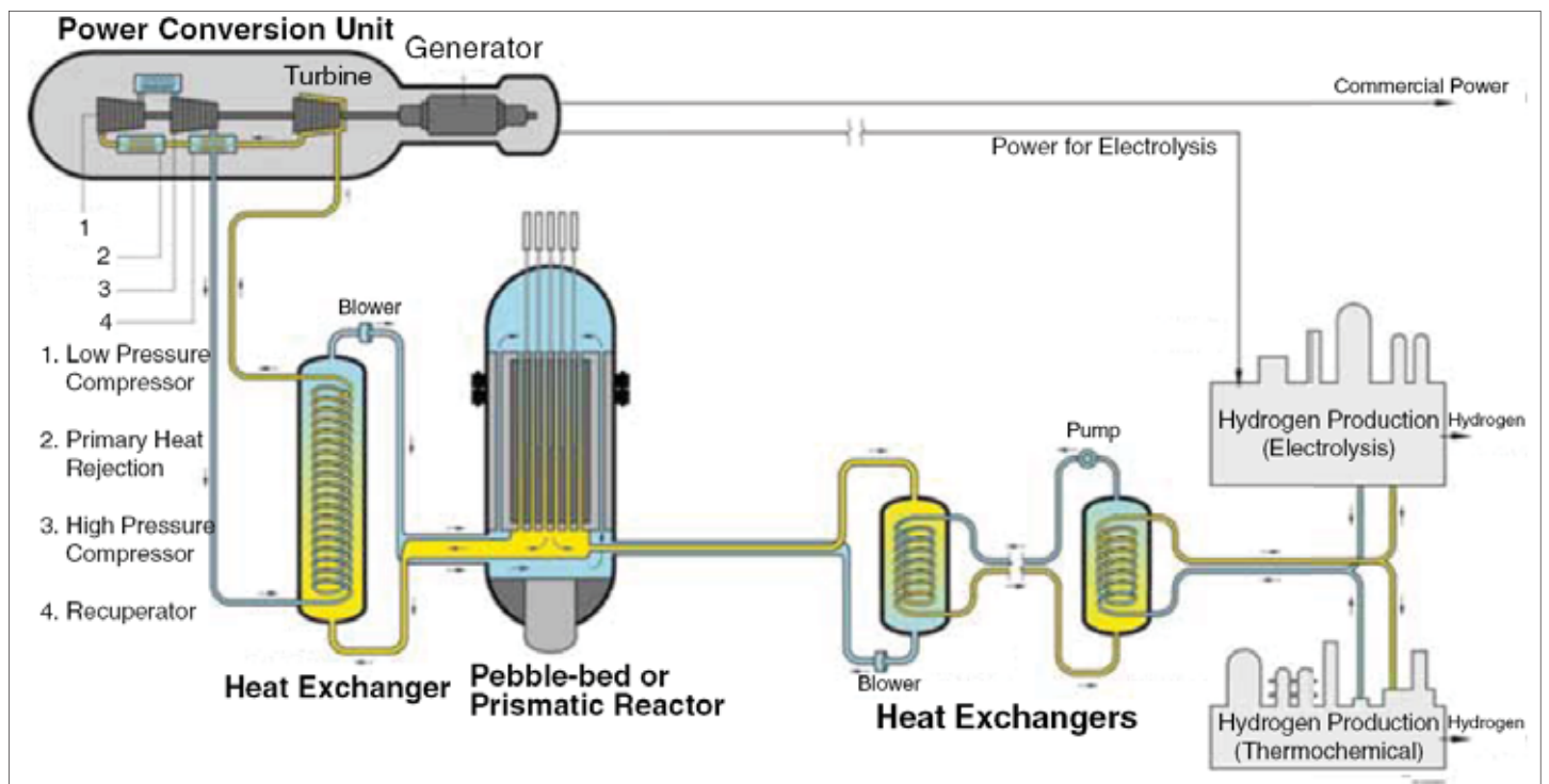
FIGURE 1 Heat transfer from a nuclear reactor.
