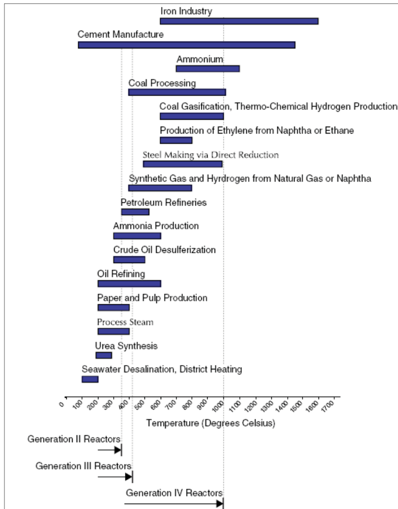
FIGURE 3 Comparison of common industrial-process heat-temperature requirements, with nuclear-reactor temperatures. 7
